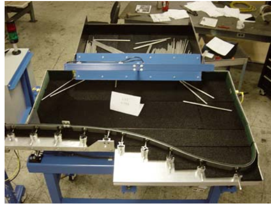
F2148 w/ Pan Feeder Hopper Includes pneumatic flow gate
