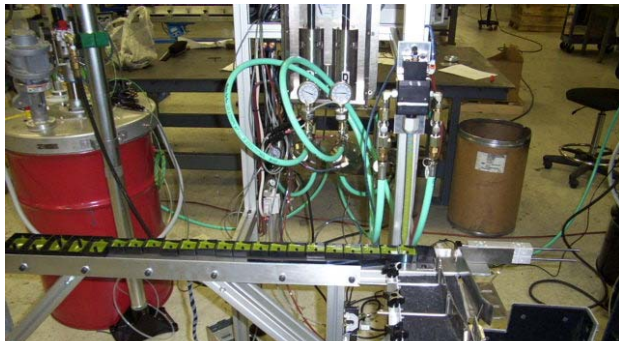
Electronic Part - Precision Feeding to OEM Substrate Dispenser
