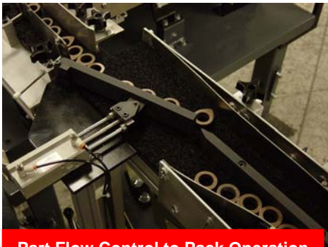
Part Flow Control to Pack Operation
